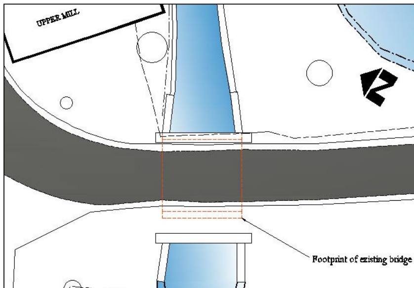
Plan showing widened replacement bridge
